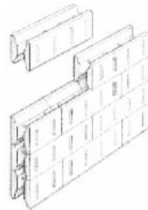
Figure 3.8: Insulated concrete form Source: Winter Panel Corporation
