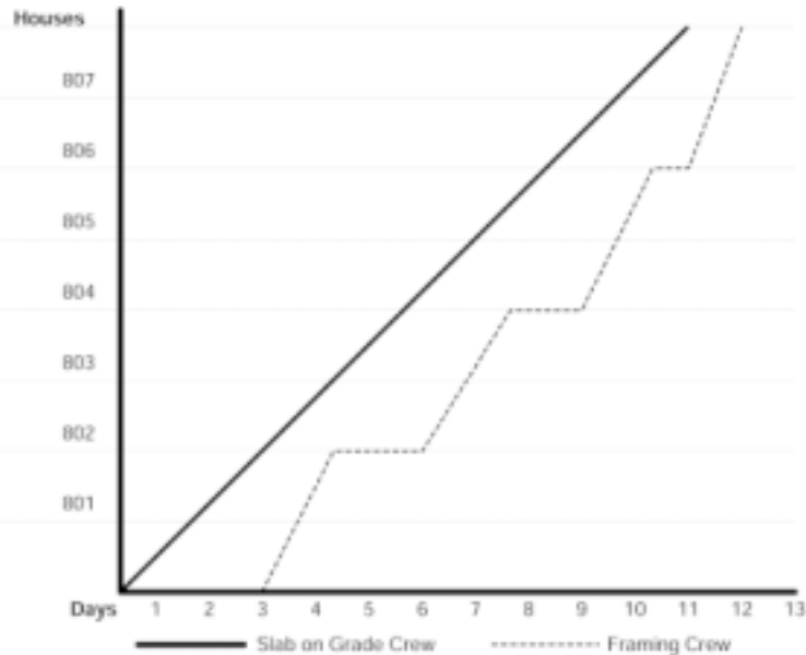
Figure 3.6: Linear scheduling graph of ideal production rate, actual start, and finish dates for framing.
