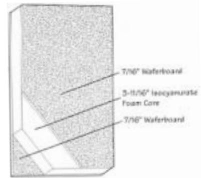
Figure 3.7: Structural insulated panel Source: Winter Panel Corporation
