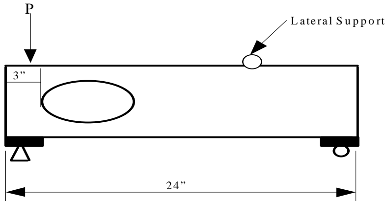
Figure 6 - ETF Web Crippling Test Setup
