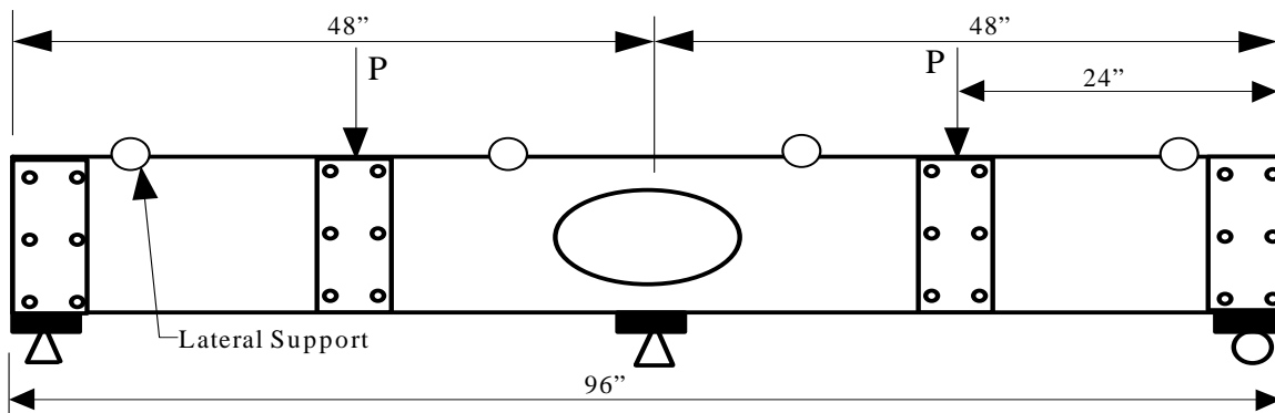
Figure 5 - Combined Bending and Shear Test Setup
