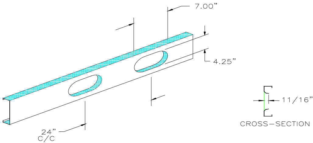
Figure 1 - Joist with 8-inch Web Depth
