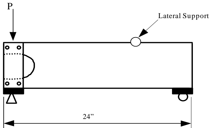
Figure 8 - Stiffened ETF Web Crippling Test Setup
