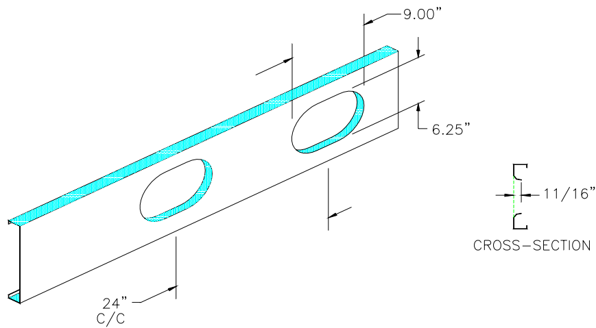
Figure 2 - Joists with 10-inch and 12-inch Web Depths
