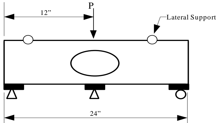
Figure 7 - ITF Web Crippling Test Setup
