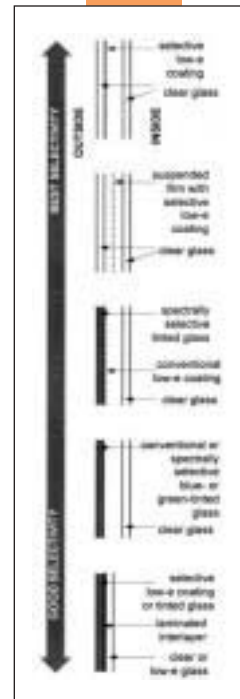
Fig. 4-23 National Fenestration Rating Council (NFRC) labeling system.
