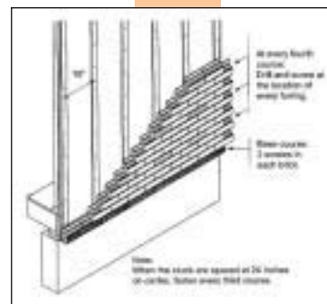
Fig. 4-20 Mortarless brick veneer installation. Illustration from Novabrik installation guidelines.
