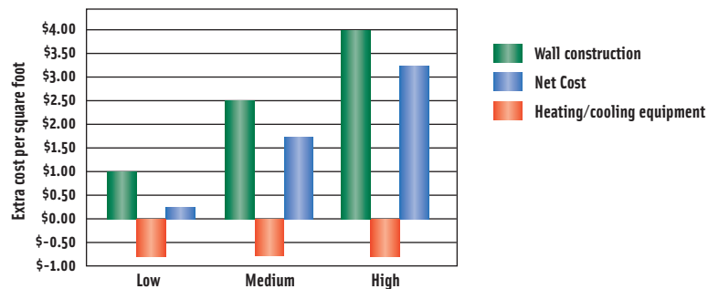
Total Costs of Construction with ICFs
