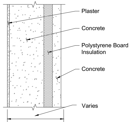
Typical sandwich panel (SP-typ)
