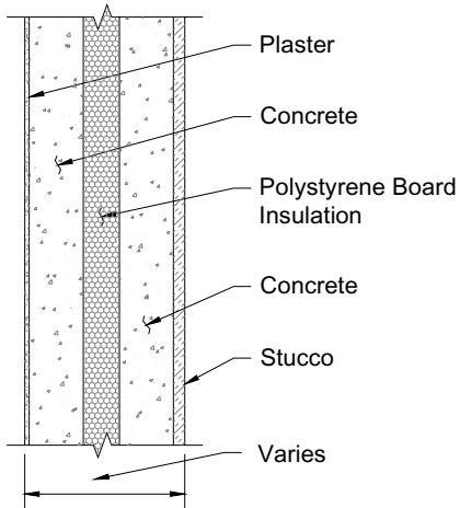
Engineered sandwich panel (SP-eng)
