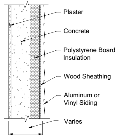
Exterior insulation (CIP ext. insul.)
