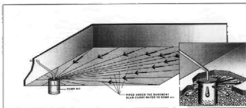
FIGURE 5. INTERIOR RADIAL SUMP SYSTEM WITH SUMP PUMP
