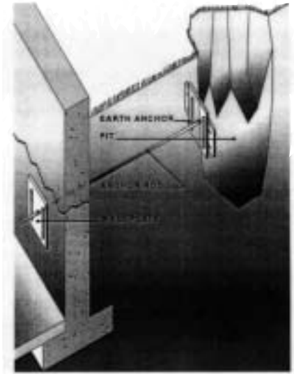
EARTH ANCHOR
