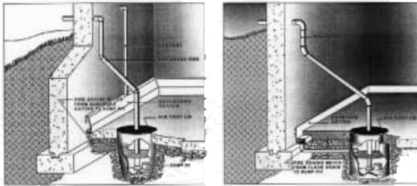
FIGURE 4. INTERIOR BASEBOARD DRAINAGE SYSTEMS
