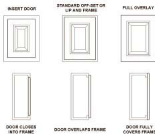
INSET, STANDARD OFFSET, AND FULL OVERLAY DOORS
