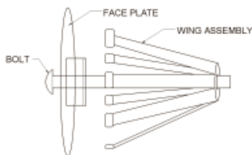
WINGIT FASTENER IN OPEN AND CLOSED POSITIONS
