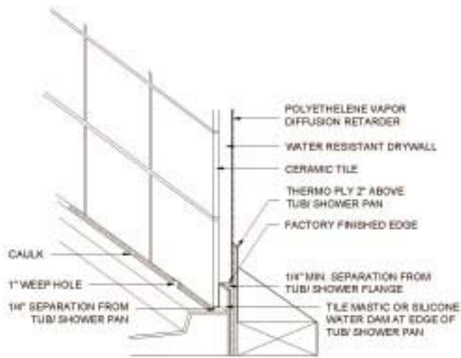
ONE-INCH WEEP HOLE IN CAULK WITH SUBSTRATE HELD OFF TUB/SHOWER FLANGE
