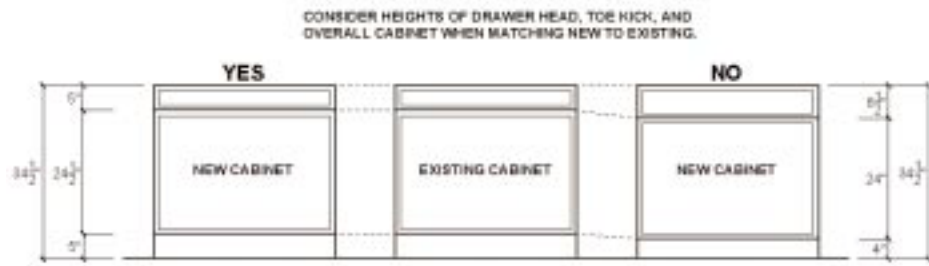
DRAWER AND TOEKICK HEIGHTS IN SUPPLEMENTARY CABINETS
