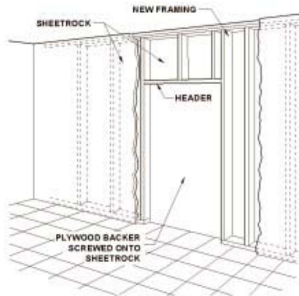
NEW FRAMING TO RECESS REFRIGERATOR INTO WALL
