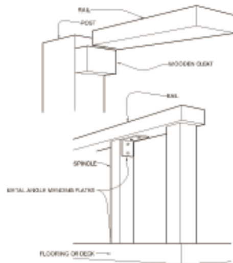
WOOD RAIL SUPPORT
