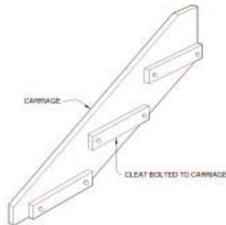
BOLTED CLEATS ON CARRIAGE
