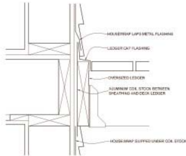
FIGURE 2 LEDGER FLASHING
